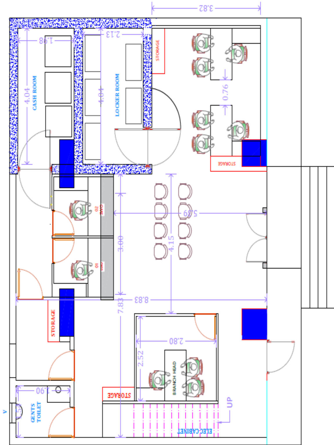
HIRA WADI GROUND FLOOR OPTION
