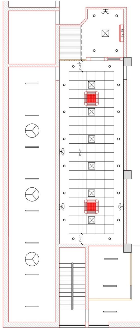
CEILING PLAN
