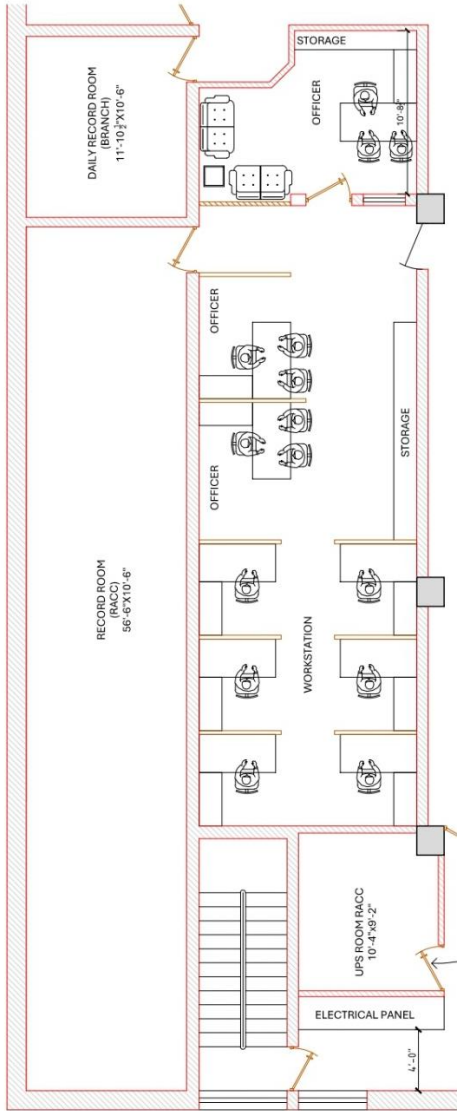
LAYOUT PLAN
