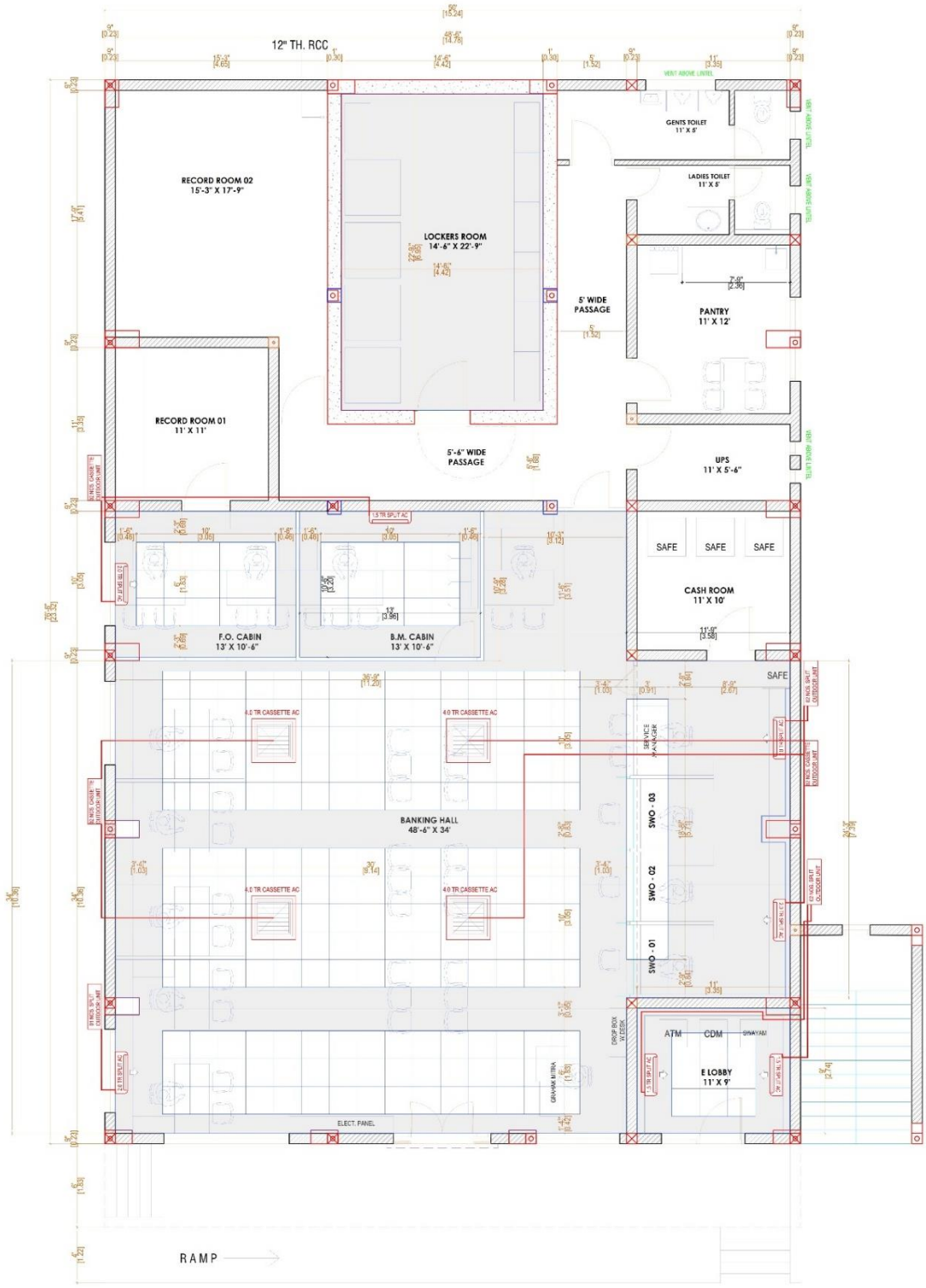
FALSE CEILING & AC LAYOUT
