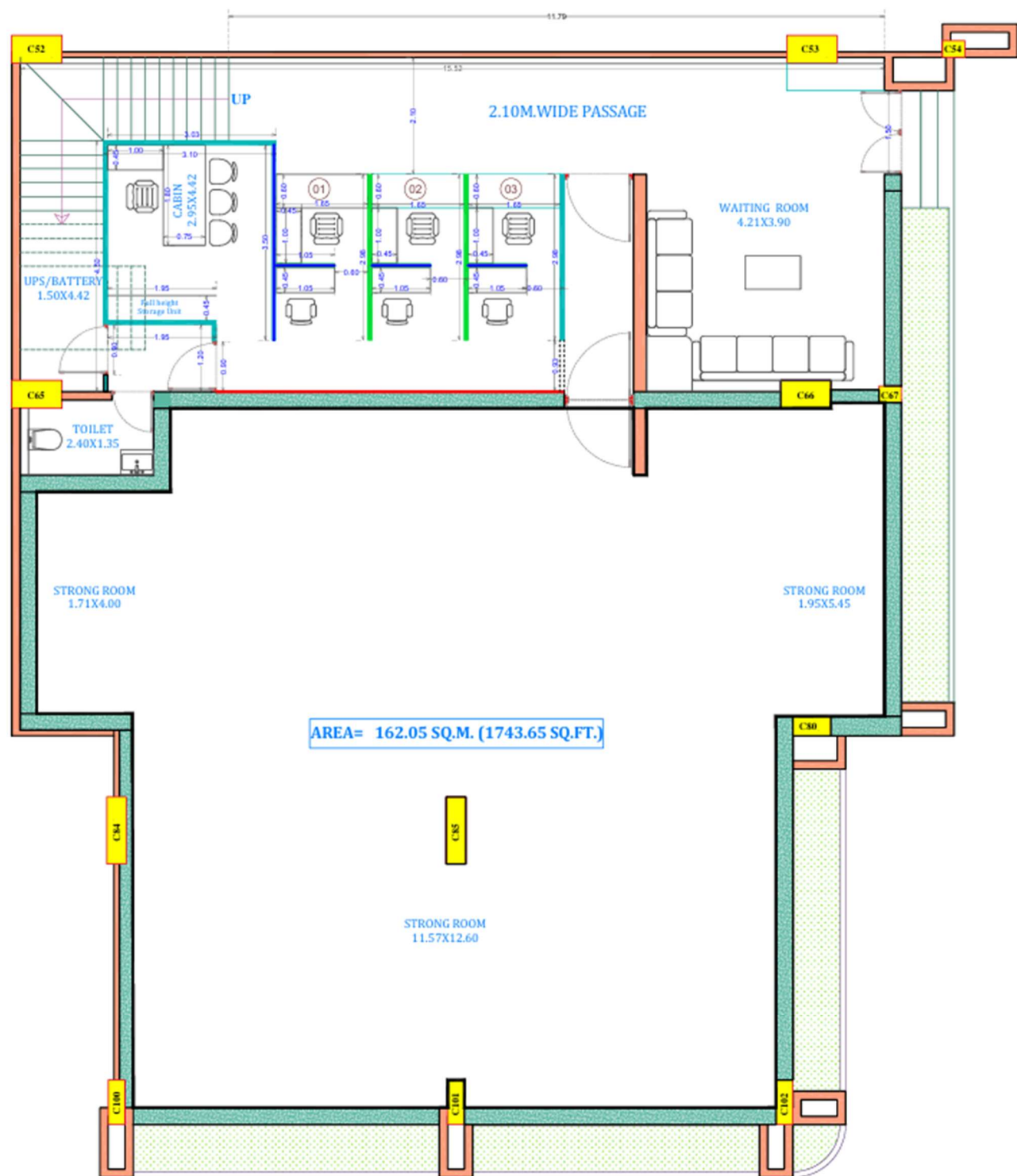
FURNITURE LAYOUT (GROUND FLOOR PLAN)
