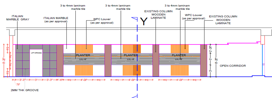
ELEVATION "B"
