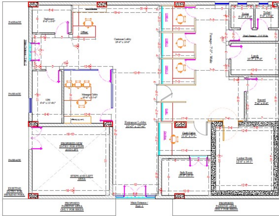
Proposed Floor plan - SBI - Uppal Branch
