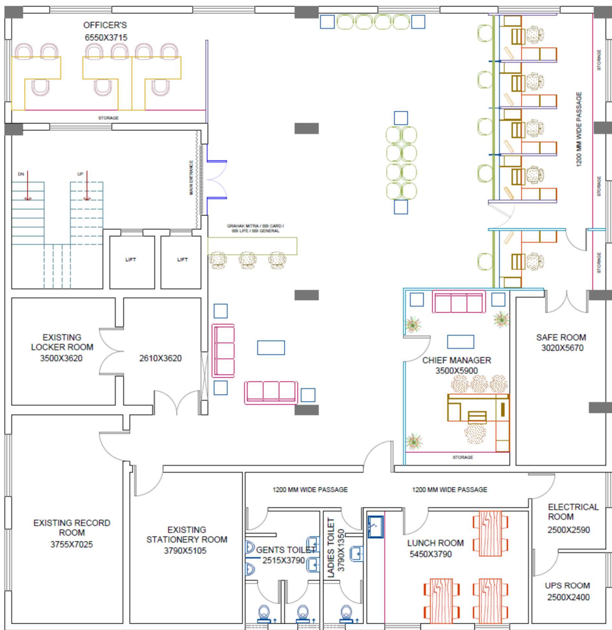
SCHEMATIC PLAN
