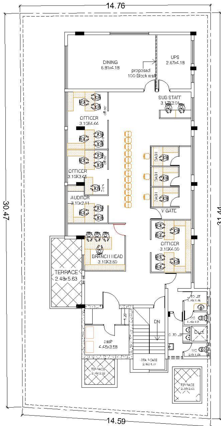
PROPOSED INTERIOR FIRST FLOOR PLAN AREA-2791.90.00 SFT
