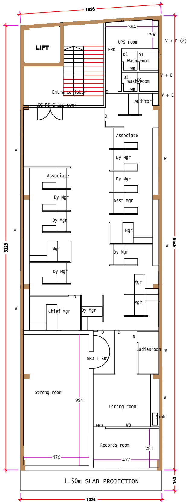
AMCC MANNARKKAD - FIRST FLOOR PLAN
