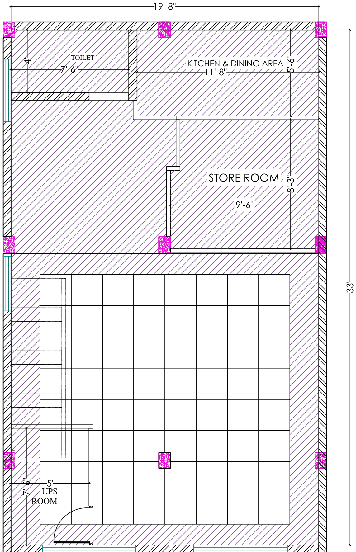
FALSE CEILING LAYOUT -FIRST FLOOR
