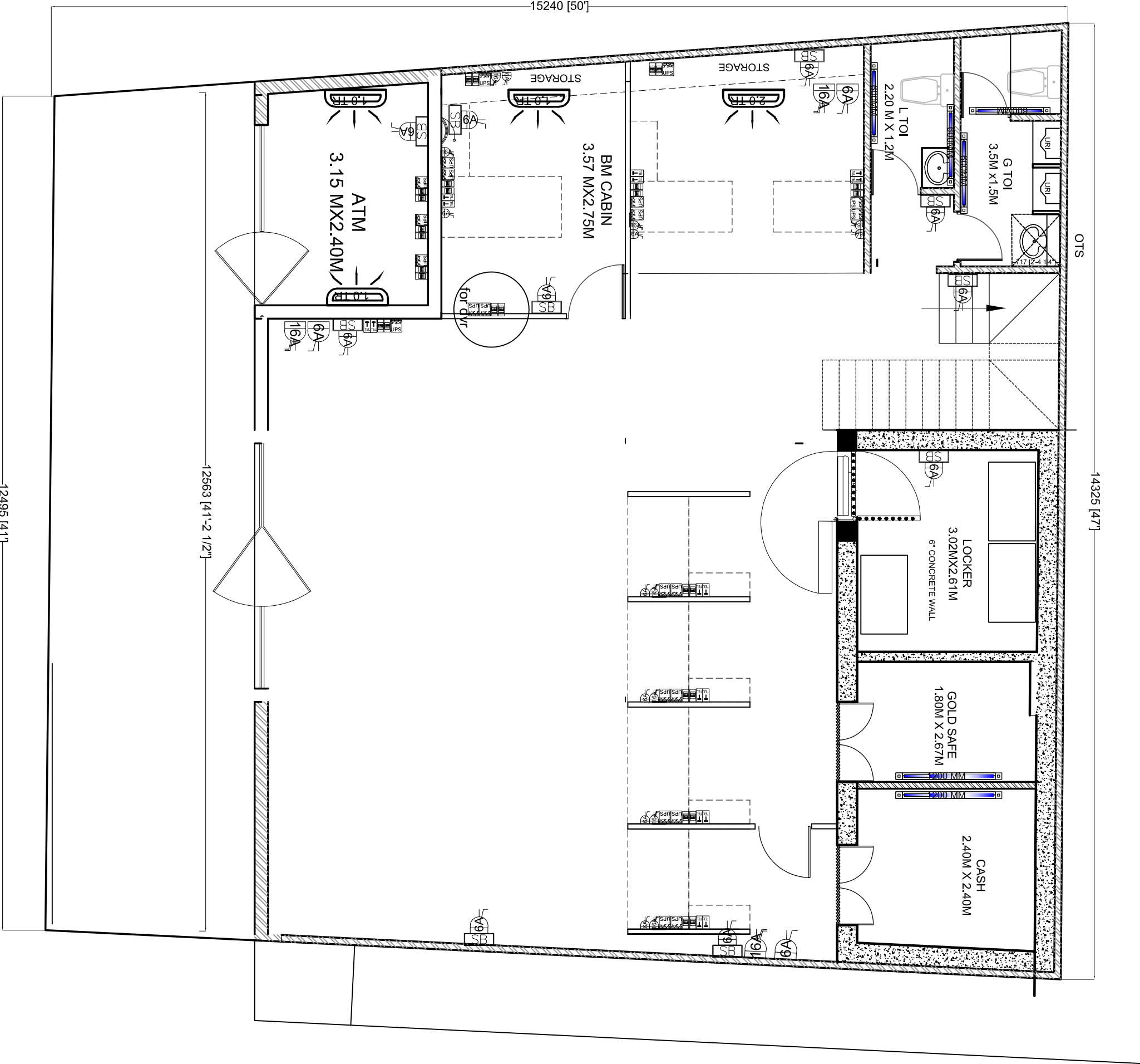
PROPOSED G FLOOR ELECTRICAL LAYOUT
