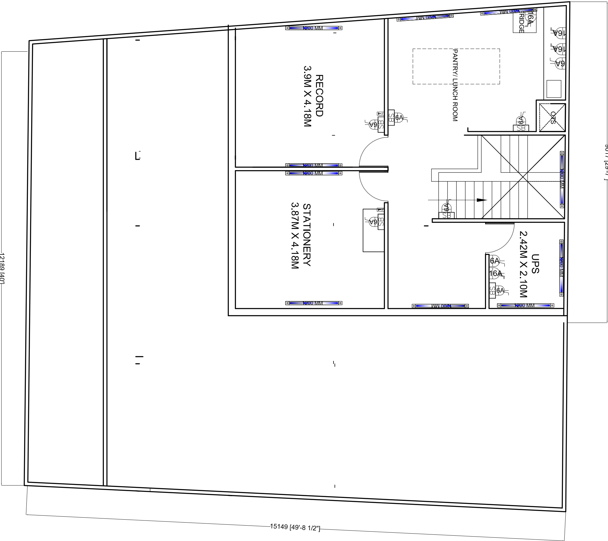
PROPOSED F FLOOR ELECTRICAL LAYOUT
