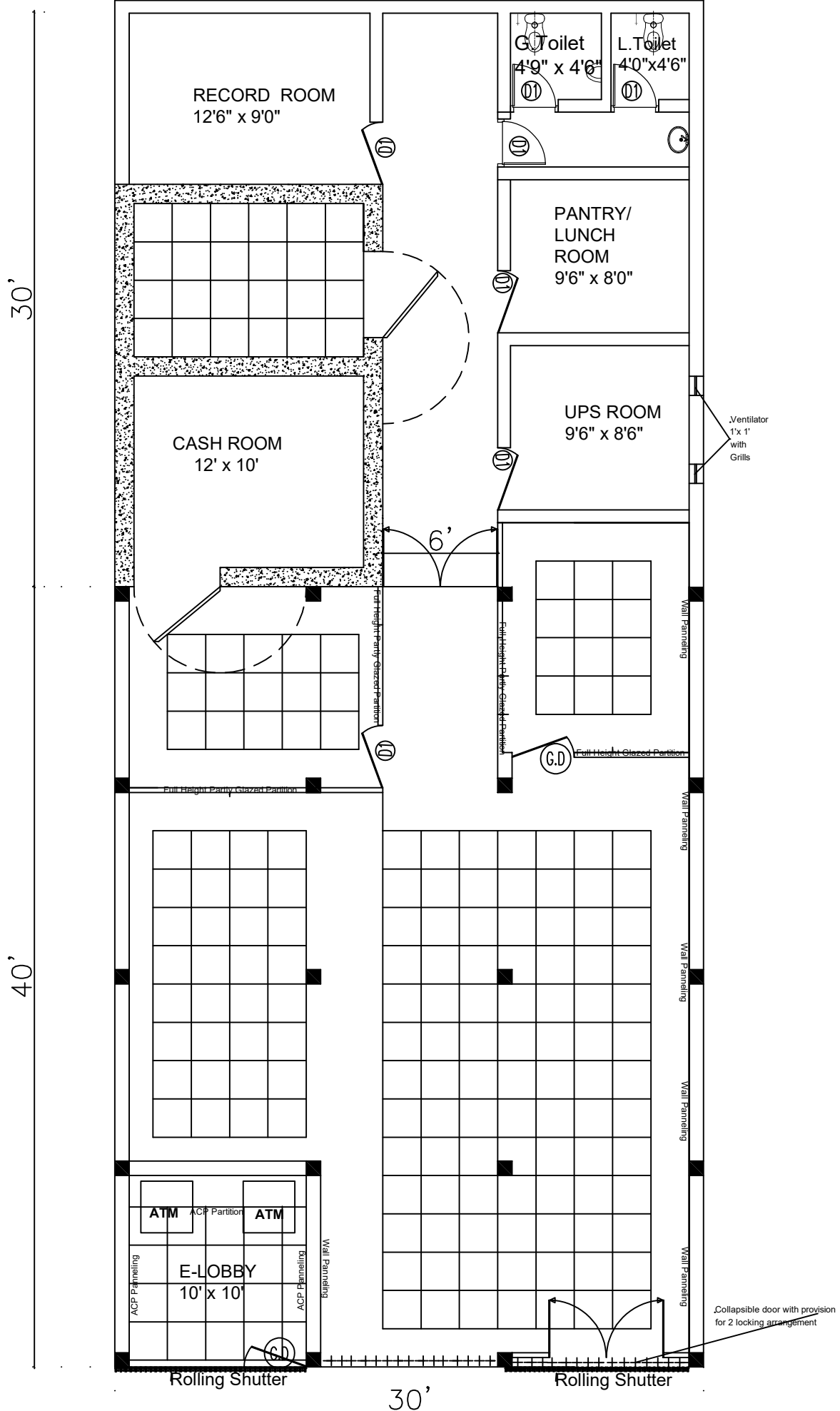
FALSE CEILING LAYOUT PLAN FOR SBI BRANCH, ALDUR
